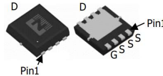
DFN3*3
